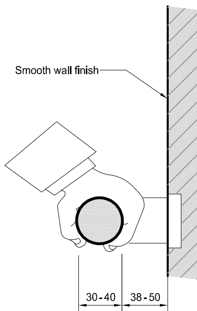
Figure 4.2.9.1: Grab Bar
