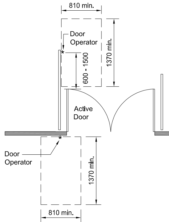
Figure 4.1.6.14: Power Door Operator Locations for Double Doors with Guardrails Opening into Path of Travel
