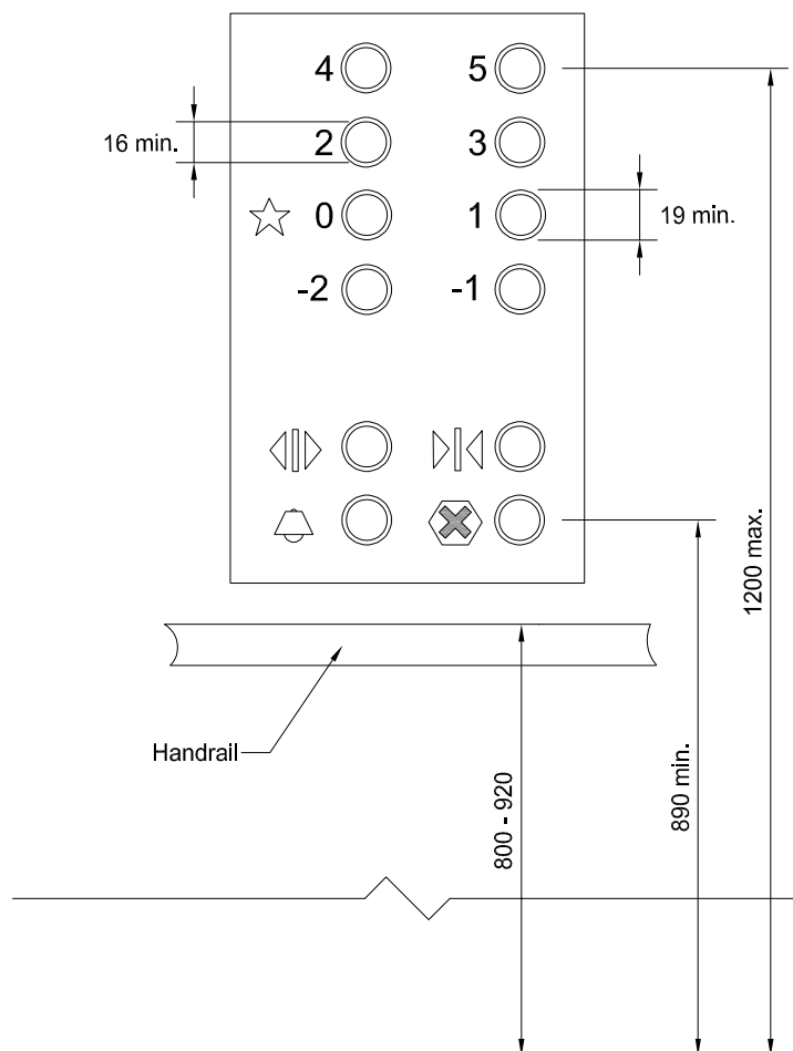
Figure 4.1.14.2: Control Panel
