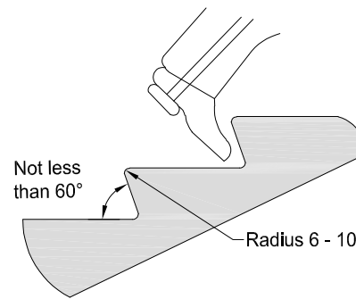
Figure 4.1.11.3: Raked Riser
