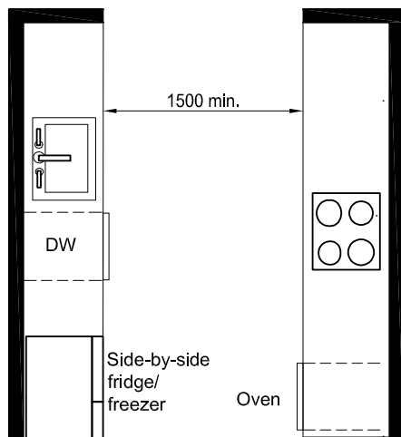
Figure 4.3.17.1: Pass-Through Kitchen
