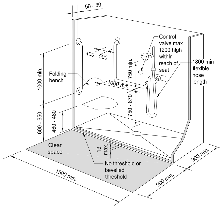
Figure 4.2.8.1: Shower Stall
