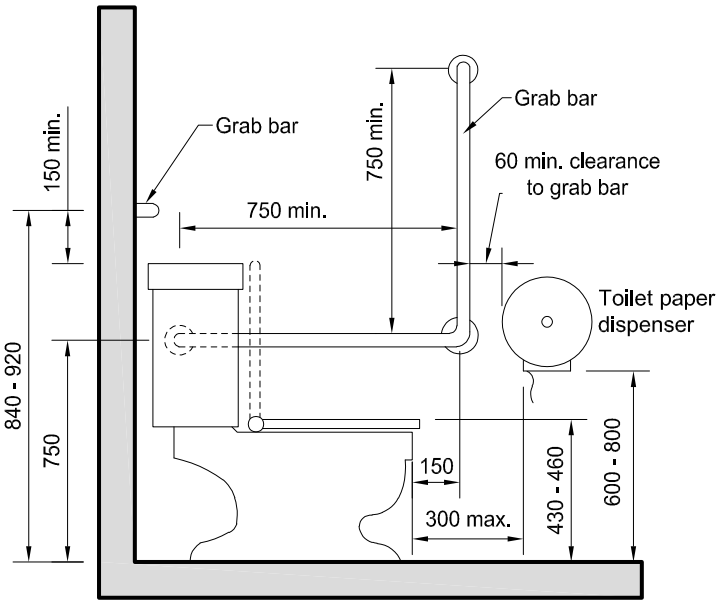
Figure 4.2.3.1: Accessible Toilet and Grab Bar Configuration
