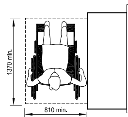
Figure 4.3.7.3: Parallel Approach
