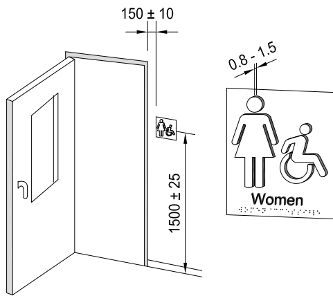
Figure 4.4.6.3: Tactile Signage
