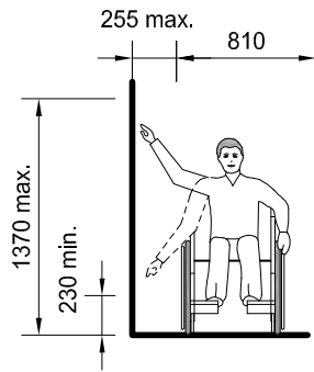
Figure 4.1.1.11 Side Reach
