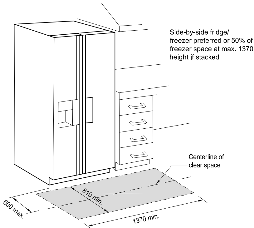
Figure 4.3.17.8: Fridge/Freezer
