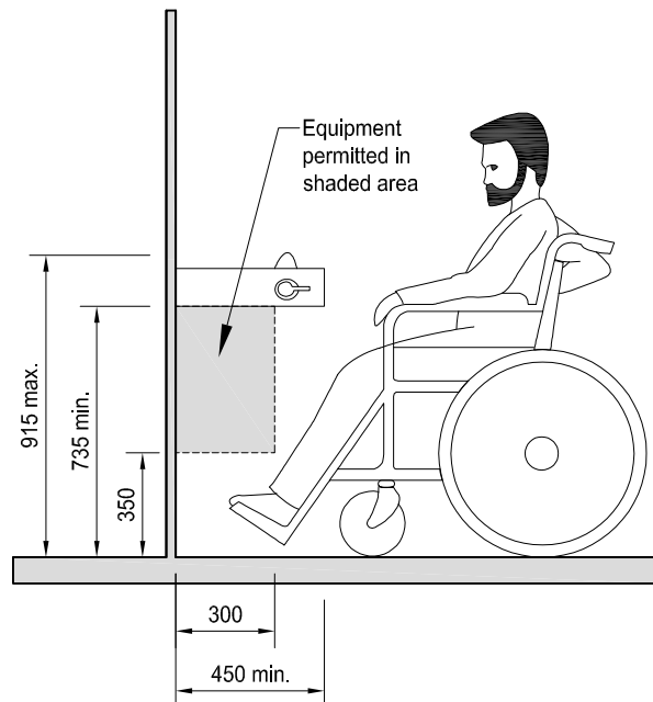
Figure 4.3.1.3: Clearances
