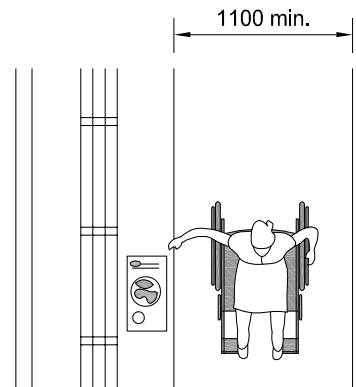
Figure 4.5.4.2: Aisle Width
