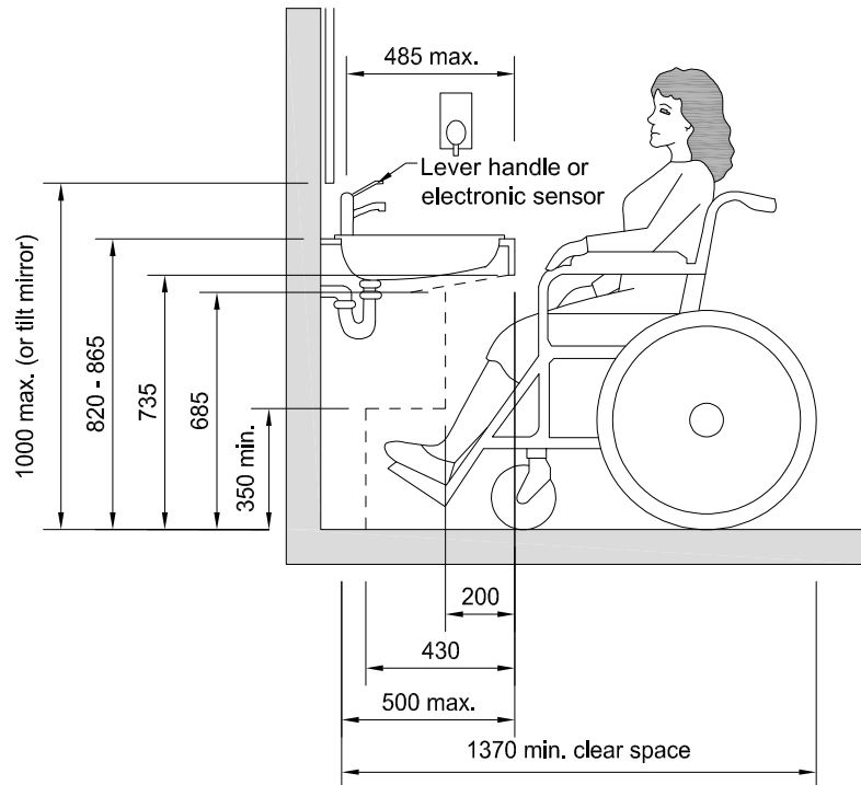
Figure 4.2.4.1: Lavatory Criteria
