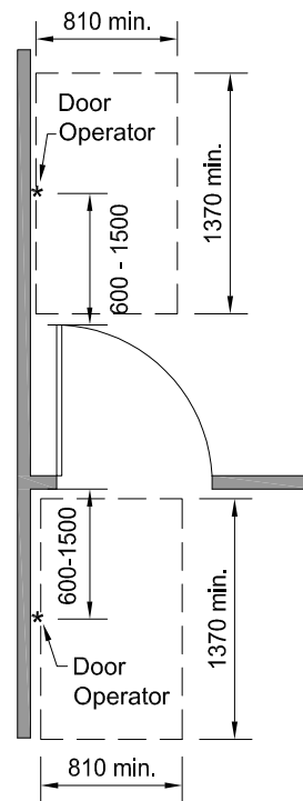
Figure 4.1.6.9: Power Door Operator Locations for Single Door Adjacent to Wall
