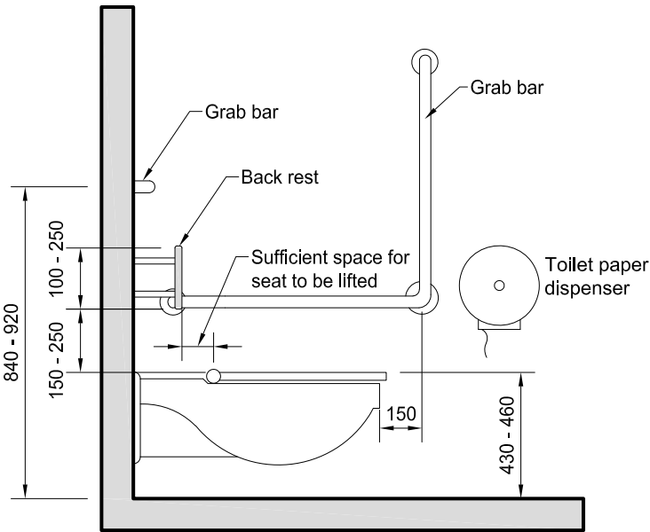
Figure 4.2.3.2: Accessible Wall Hung Toilet with back Rest
