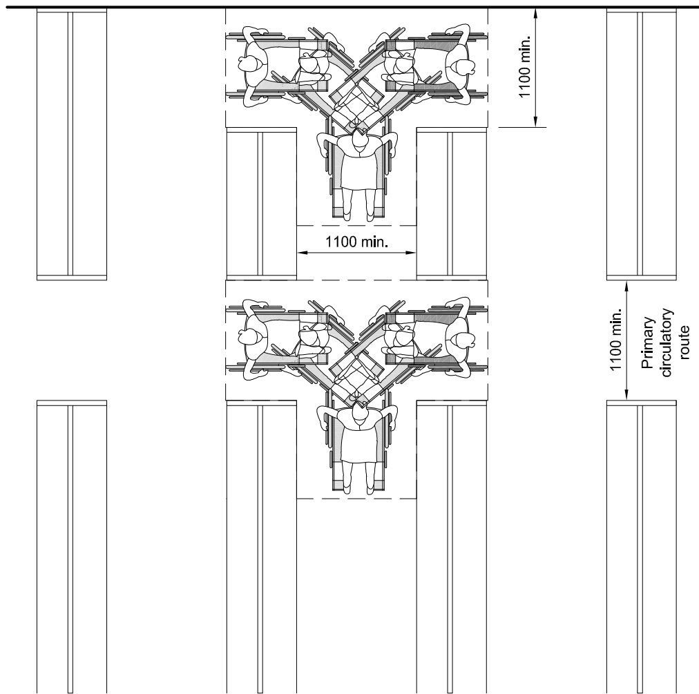
Figure 4.5.6.1: Aisle Widths
