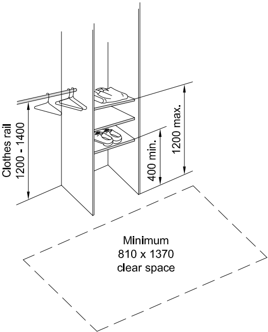
Figure 4.5.9.2: Closet Dimensions
