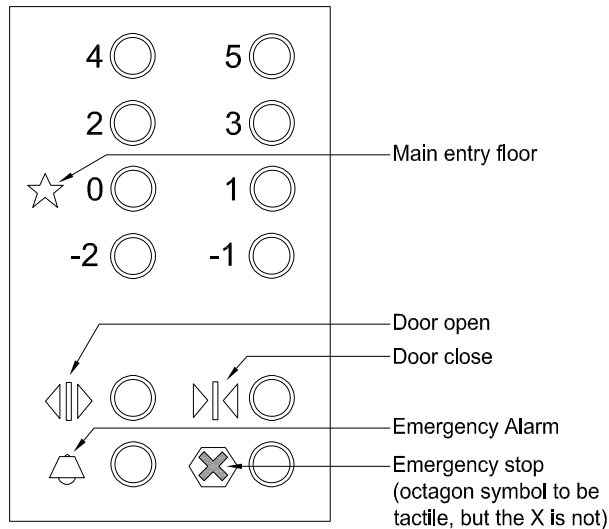
Figure 4.1.14.4: Tactile Elevator Button Symbols
