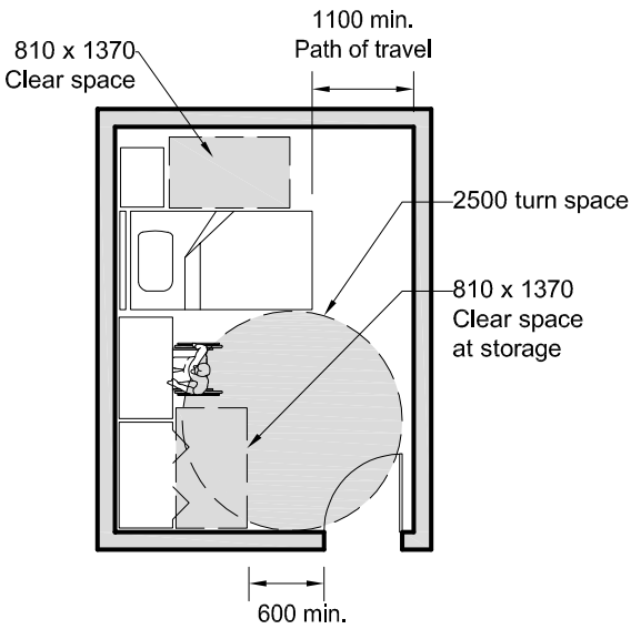
Figure 4.5.9.3: Residence Layout and Dimensions
