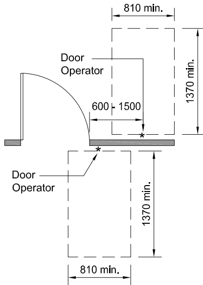
Figure 4.1.6.8: Power Door Operator Locations for Single Door
