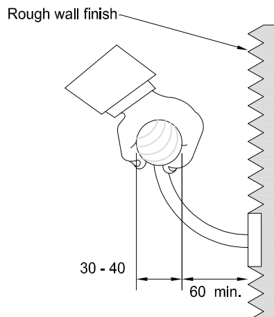
Figure 4.1.12.2: Handrail at Rough Wall
