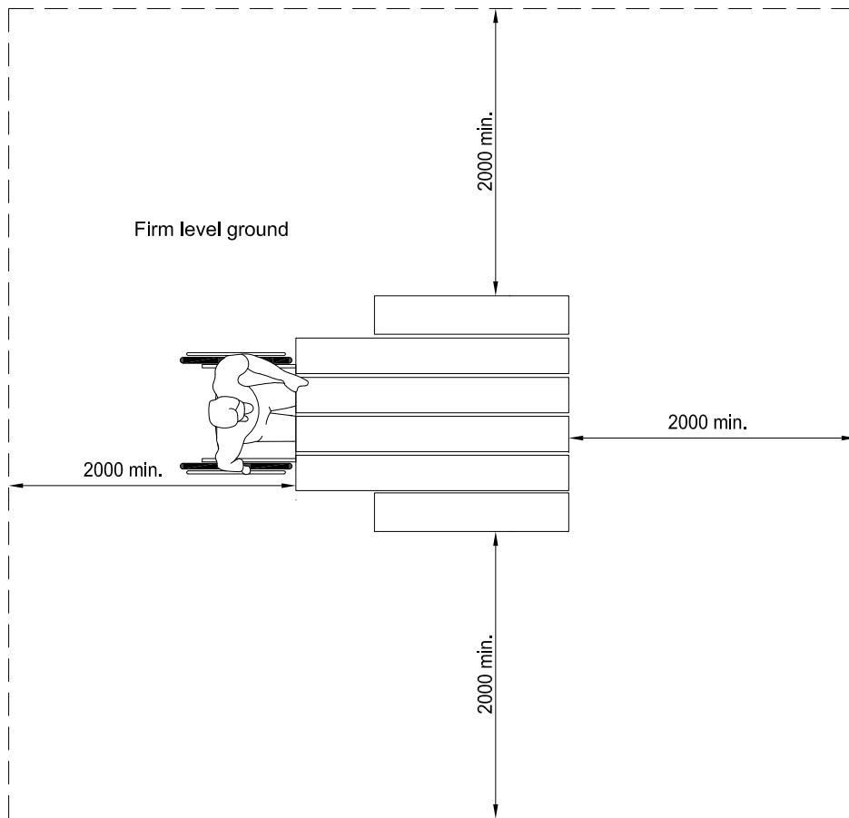
Figure 4.3.14.2: Accessible Tables
